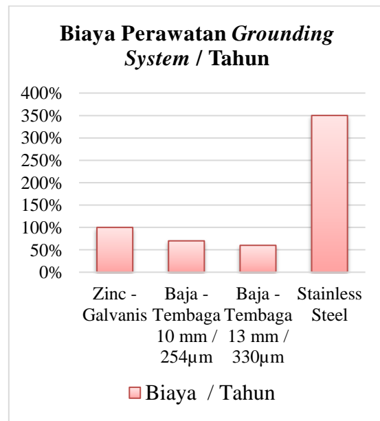
Gambar 5. Perbandingan Biaya Perawatan Grounding Rod.
