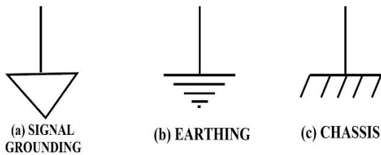
Gambar 2. Simbol Grounding
