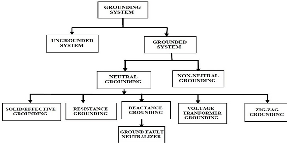
Gambar 1. Metode Grounding System
